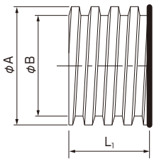
TDW350~1000
