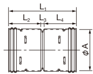
φ150, 200
